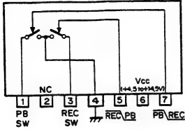
uPC1513HA (NEC) AUDIO HEAD SELECT SWITCH — PRINTED SIDE VIEW —
